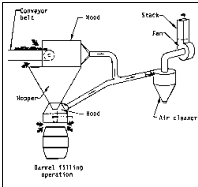
Figure 19-1. Typical Local Exhaust Ventilation system. (Source: McDermott, 2000.)
