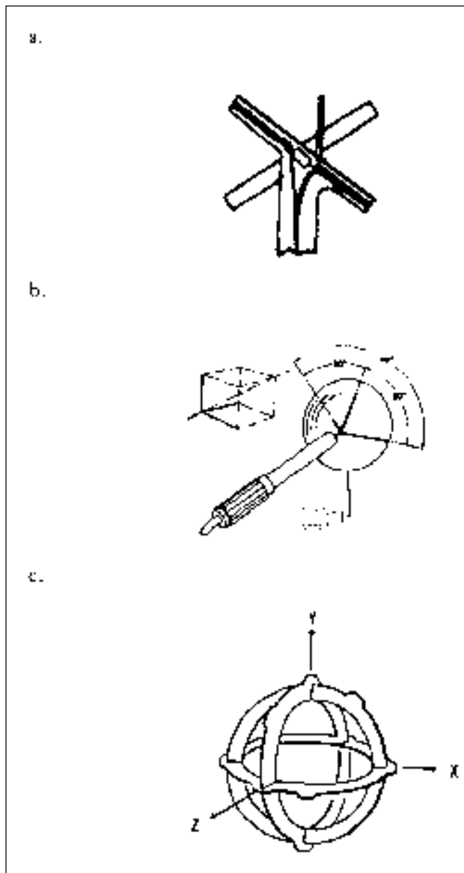
Figure 11-16. Isotropic (nondirectional) antenna arrays. a. Mutually orthogonal dipoles respond to electric fields (Holaday Industries HI 3102 probe). b. Mutually perpendicular array of thermocouples (Loral/Narda 8621 series probes). c. Mutually perpendicular magnetic field loops.
