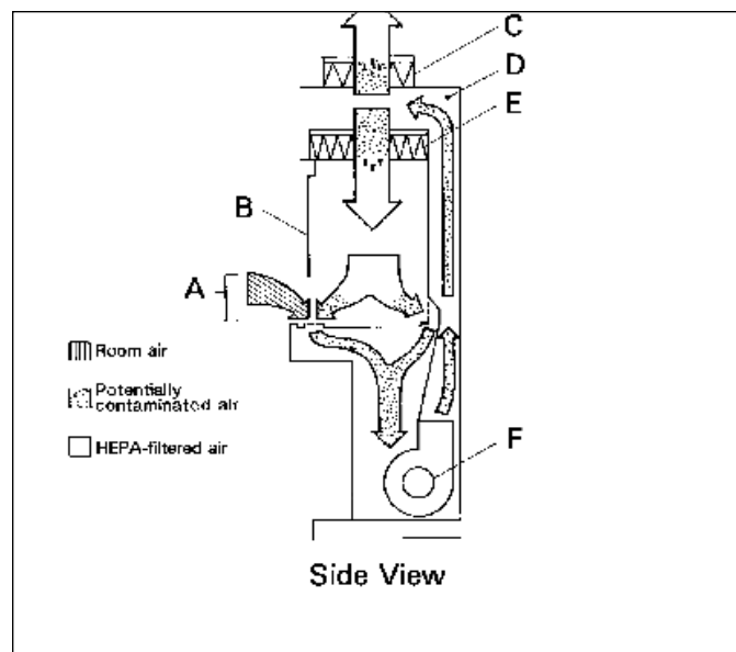
Figure 14-2a. Class II, type A biological safety cabinet. A. front opening, B. sash, C. exhaust HEPA filter, D. rear plenum, E. supply HEPA filter, F. blower. (Reprinted from BMBL , CDC, 1999, p 207.)
