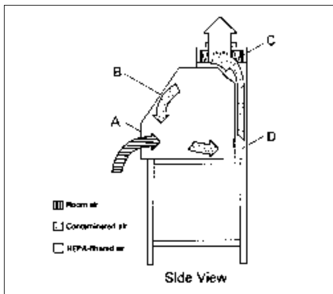
Figure 14-1. Class I biological safety cabinet. A. front-opening, B. sash, C. exhaust HEPA filter, D. exhaust plenum. (Reprinted from Biosafety in Microbiology and Biomedical Laboratories [BMBL] . CDC, 1999, p 206.)
