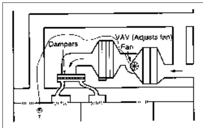
Figure 21-6. VAV HVAC system.
