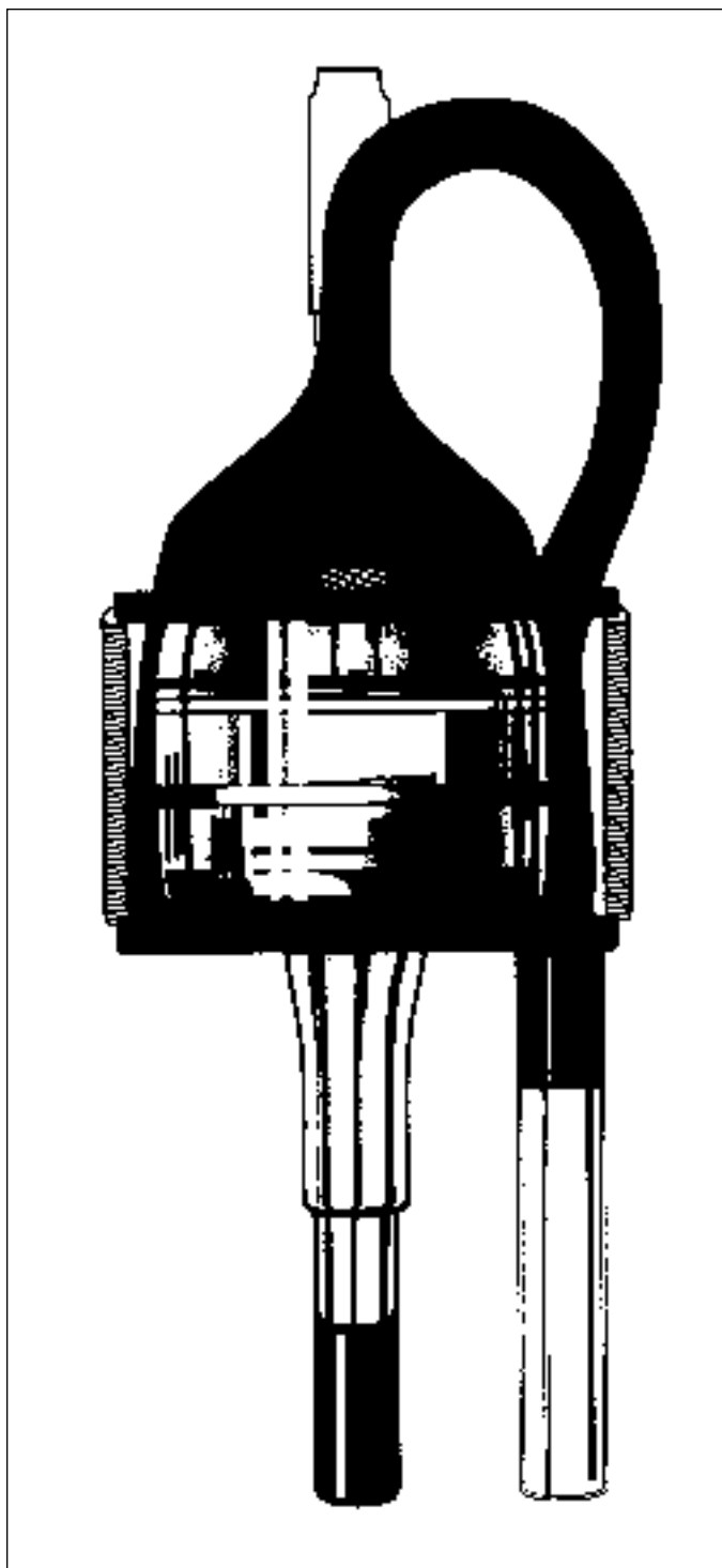
Figure 16–11. A cyclone attached to a filter cassette is used to sample for respirable dust. The filter cassette holder can be placed in the worker's breathing zone. (Courtesy SKC, Inc.)
