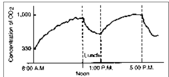
Figure 21–10. Typical carbon dioxide concentrations in today's buildings.
