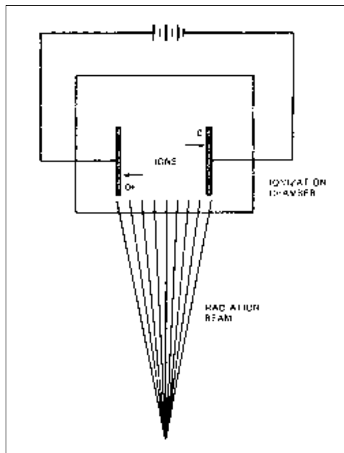
Figure 10-9. Diagram of an ionization chamber.
