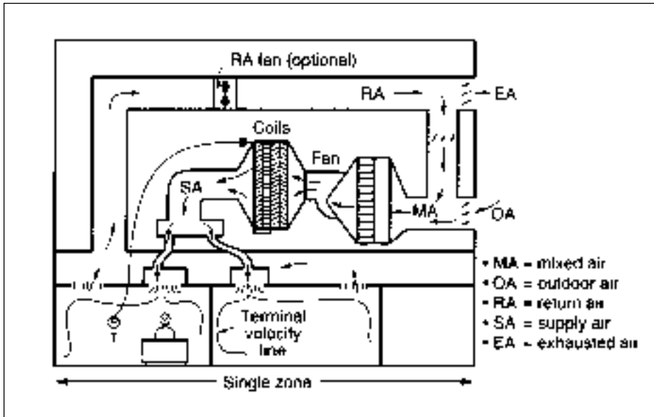
Figure 21-3. Typical single-zone constant-volume HVAC system. Note: MA = mixed air; OA = outdoor air; RA = return air; SA = supply air; EA = exhausted air. (Source: Burton, IAQ and HVAC Workbook , 1995.)
