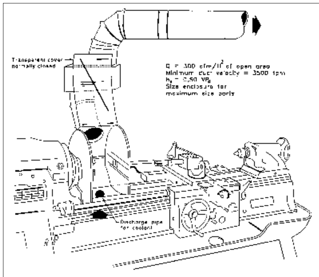
Figure 19-3. Design details for an enclosure from the ACGIH Manual. (Source: From American Conference of Governmental Industrial Hygienists (ACGIH®). Industrial Ventilation: A Manual of Recommended Practice , 23rd ed. Copyright 1998, Cincinnati. Reprinted with permission.)
