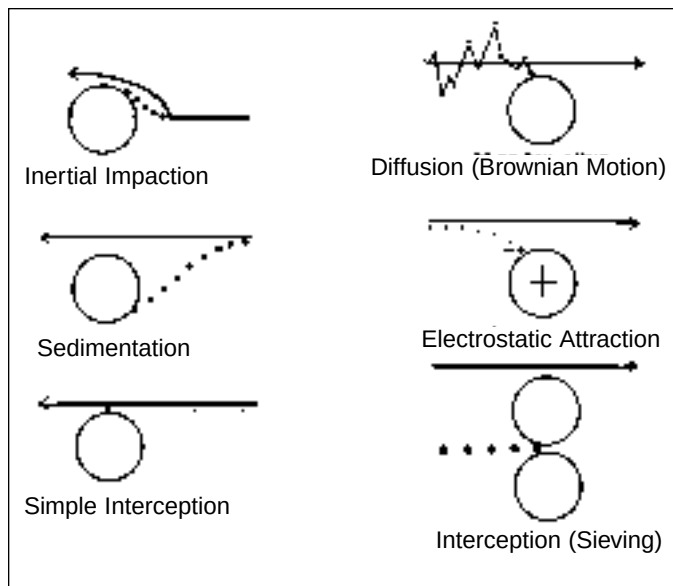
Figure 8-2. Particle deposition mechanisms.
