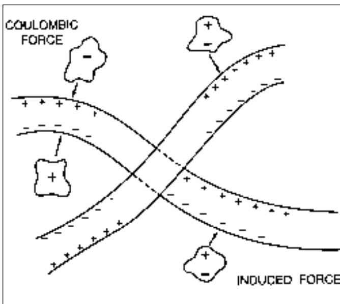
Figure 22-9. Long-range attraction of particles by the permanently charged electret fibers. A coulombic force attracts the two charged particles on the left, while a polarization force attracts the two uncharged particles on the right.
