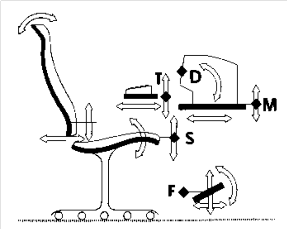
Figure 13–24. Adjustment features of a computer workstation. Key: S = seat height; T = table height; F = footrest height; D = monitor height; M = support height. (Reprinted with permission from Kroemer 2001.).
