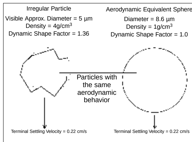
Figure 8–7. Real particle diameter and shape and aerodynamic equivalent diameter.
