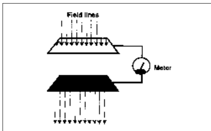
Figure 11-6. Displacement (split-plate) electric sensor used for AC field instruments in extremely low-frequency through medium-frequency regions ( >0 Hz–3 MHz). Note that field lines impinge on the upper plate, drive a current through the meter, and reemerge at the other plate. The field strength is the voltage difference between the two plates divided by the distance (V/m).
