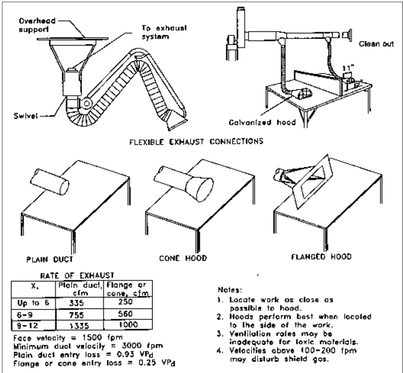
Figure 19-2. Capturing hood for welding fumes. (Source: From American Conference of Governmental Industrial Hygienists (ACGIH®). Industrial Ventilation: A Manual of Recommended Practice , 23rd ed. Copyright 1998, Cincinnati. Reprinted with permission.)
