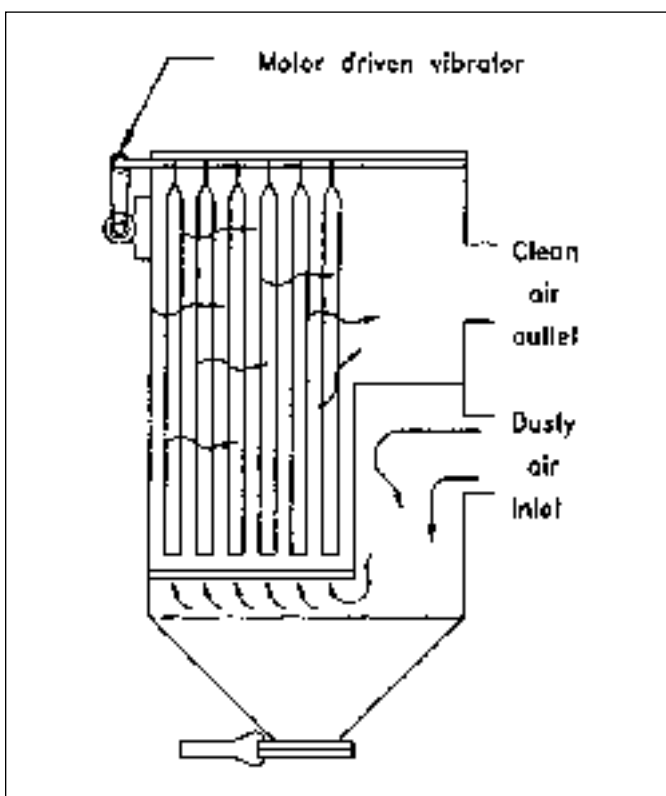
Figure 19–9. Typical baghouse air cleaner. (Source: From American Conference of Governmental Industrial Hygienists (ACGIH®). Industrial Ventilation: A Manual of Recommended Practice , 23 rd ed. Copyright 1998, Cincinnati. Reprinted with permission.)
